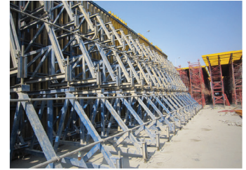
Acrow One shutter solidier
